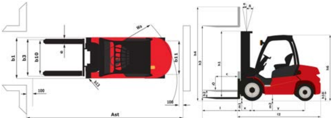
MI 35 D ST5 - Dimensional drawing
