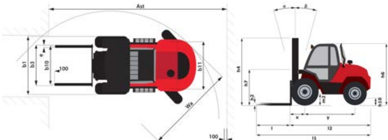
M 70-2H STG5 - Dimensional drawing
