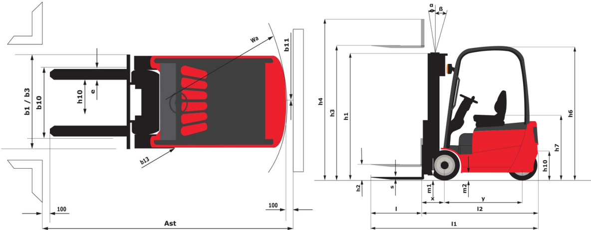
ME 450 - Dimensional drawing
