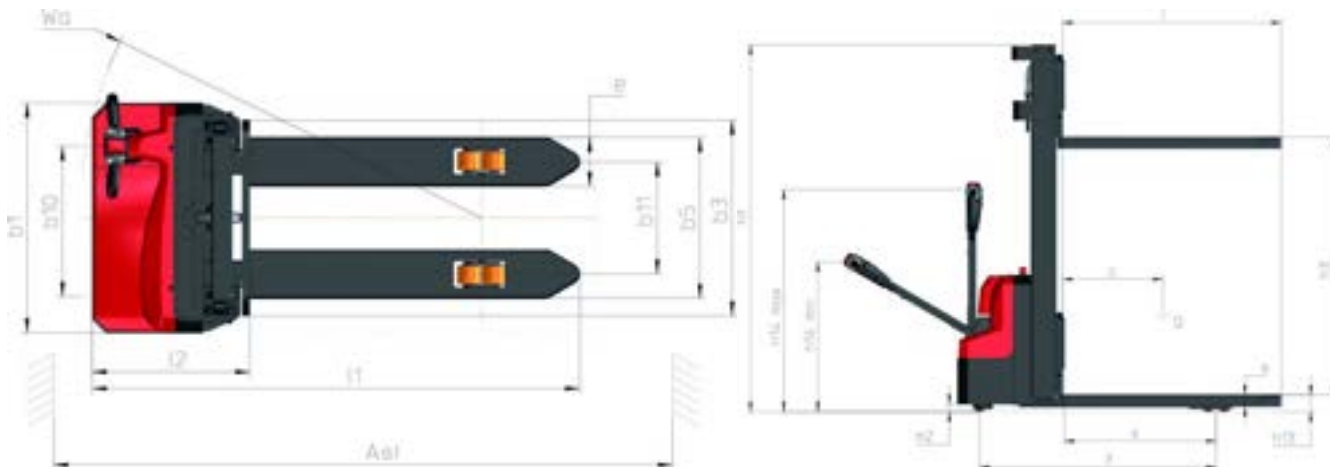
ES 112 Easy - Dimensional drawing
