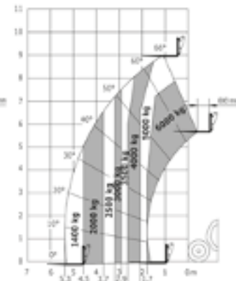
Industrial load chart standard EN1459 B Machines on tyres with forks
